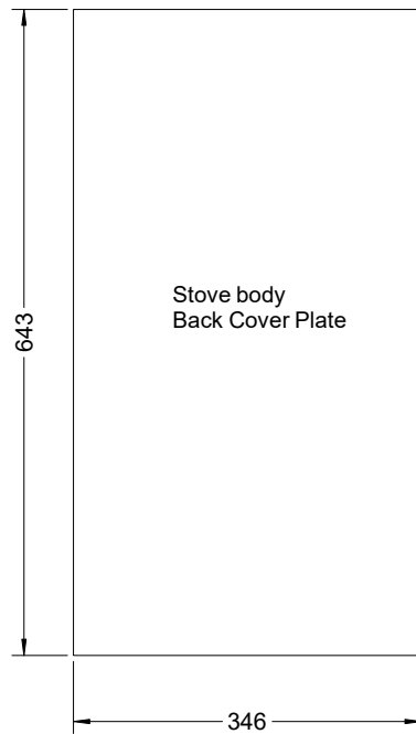
Outer Shell End Plate
